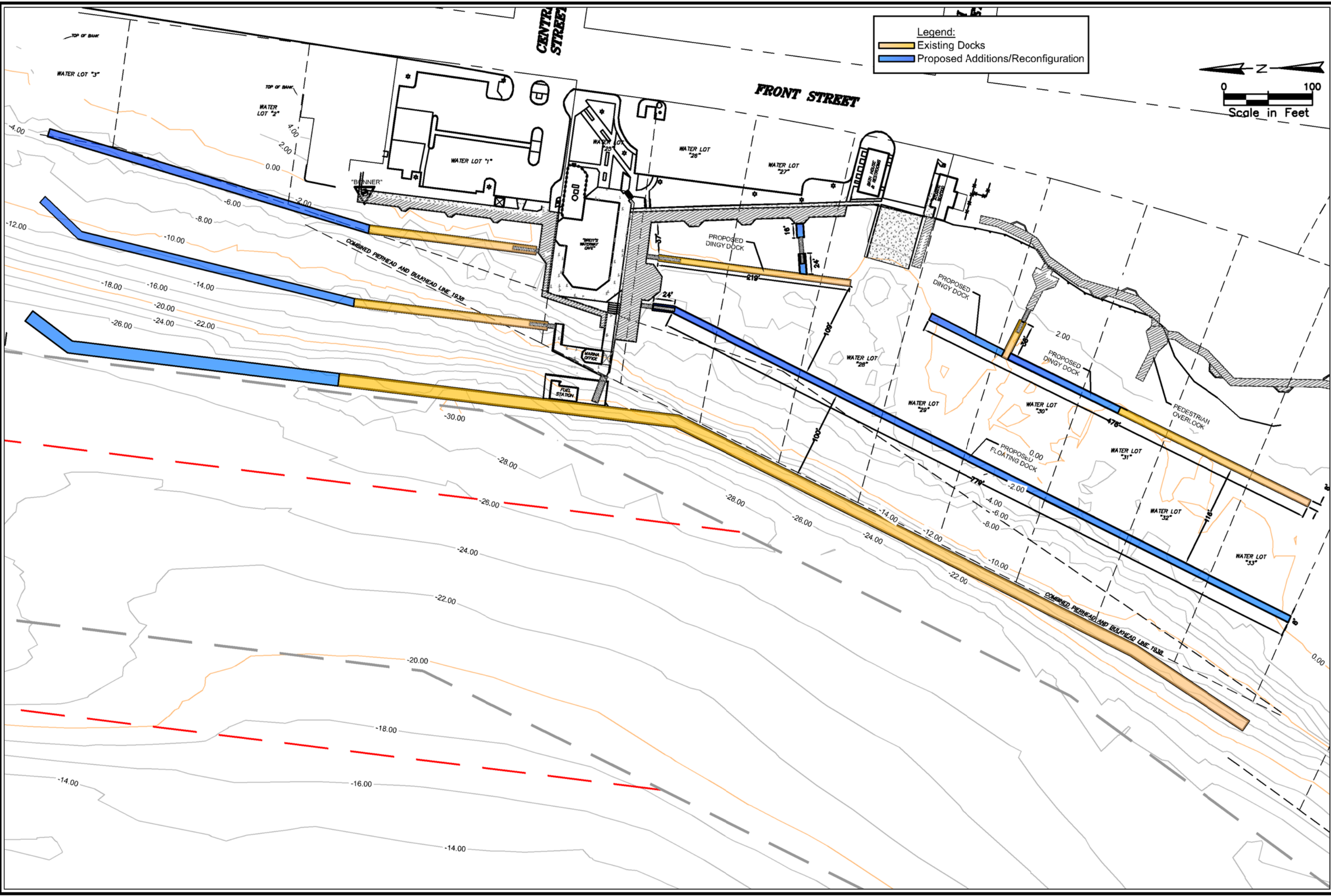
Fernandina Harbor Marina - Proposed Basin Reconfiguration Figure 2
